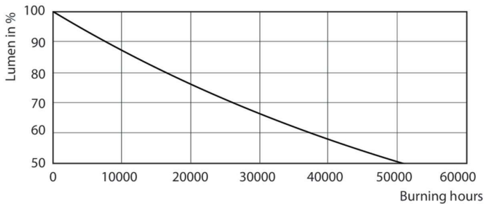
Lumen Maintenance Diagram - Master LED 4.9-50W GU10 930 36D Dim
