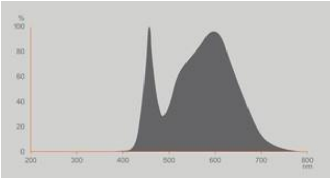
EPREL Data Spectral Diagram LEDr _6500K
